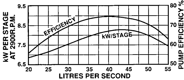
PUMP EFFICIENCY AND KW / STAGE
